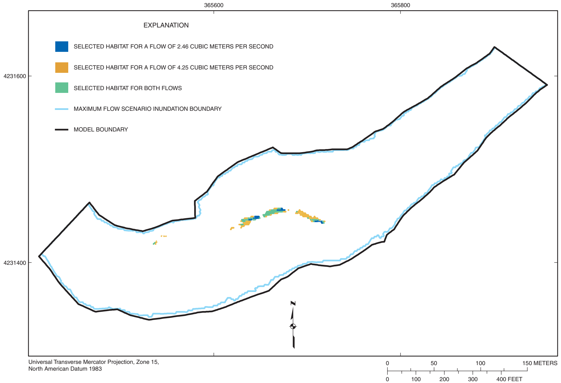
Figure 4-58. Selected habitat area distribution for habitat categories 16, 17 combined (channel catfish) at flows of 2.46 and 4.25 cubic meters per second at Marais des Cygnes River site MDC2.
